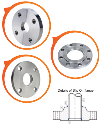
1. Slip On flange 2. Filled weld outside 3. Filled weld inside 4. Pipe
