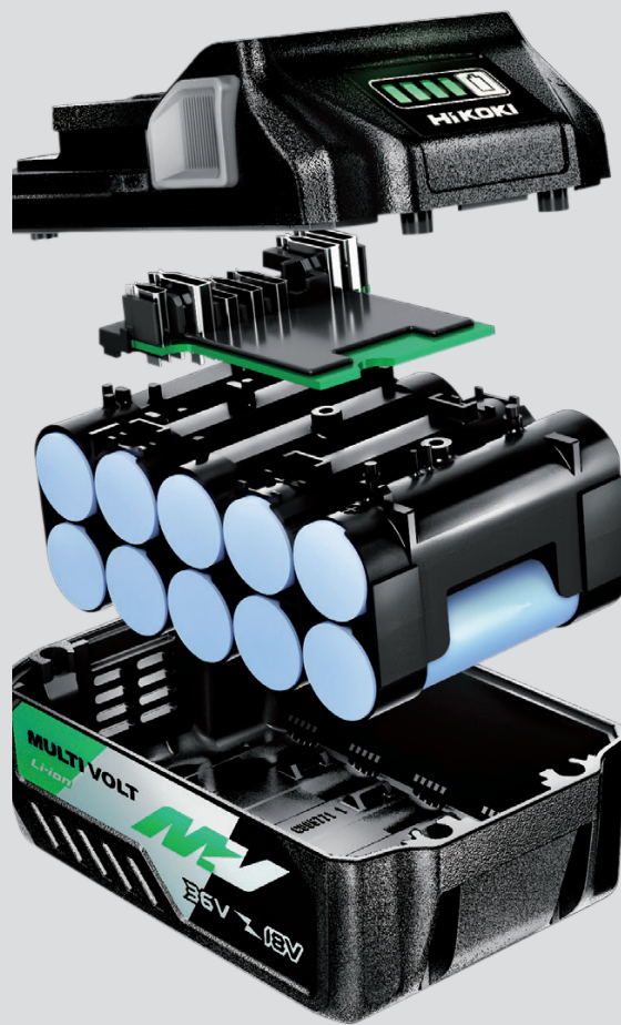
BSL36A18 / BSL36B18 MULTI VOLT Battery
